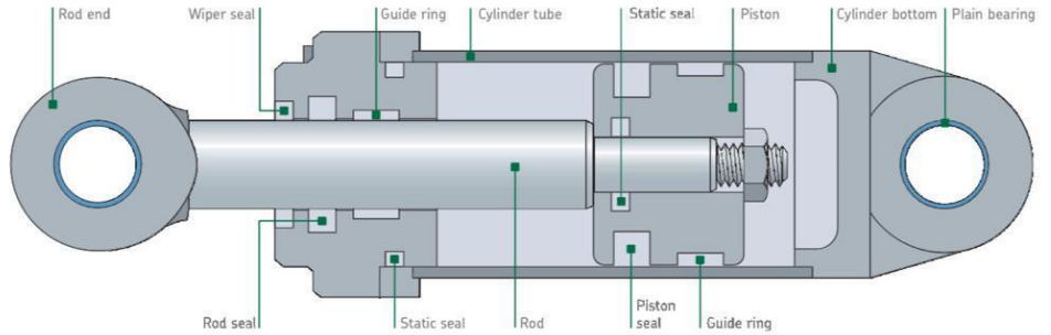
Hydraulic cylinder
